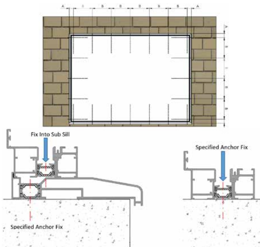
Typical outer frame installation with sub-sill
